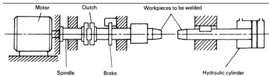
Gambar 2. Direct-Drive Friction Welding
