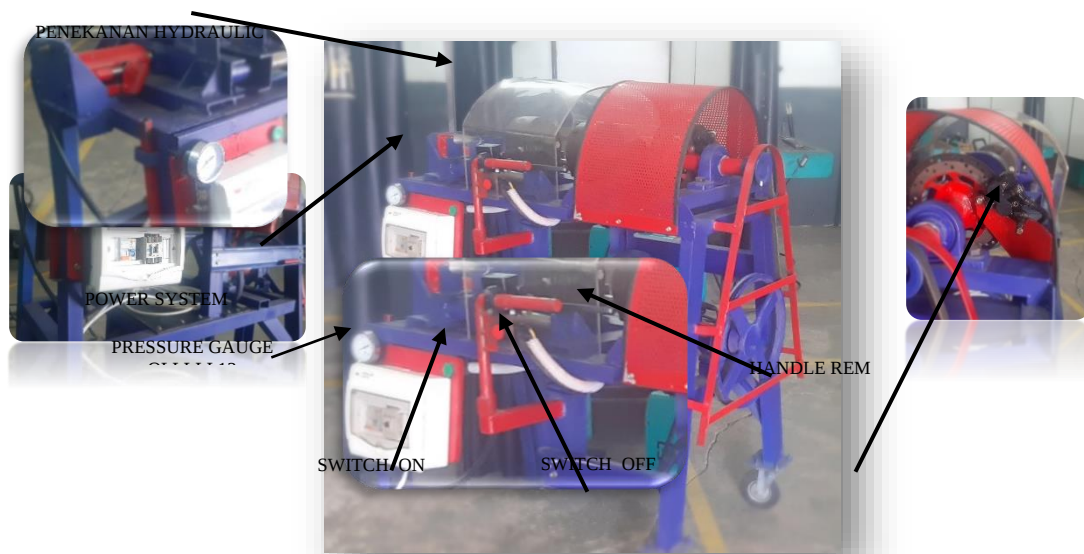
Gambar 4. Friction Rotary Welding
