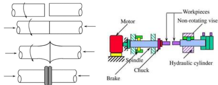
Gambar 1. Proses Kerja Friction Rotary Welding
