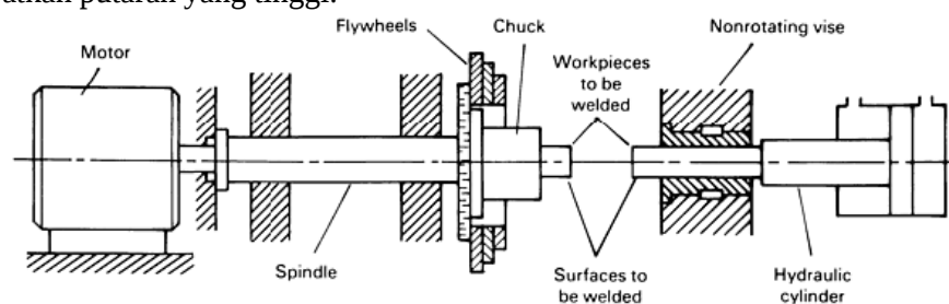
Gambar 3. Inertia-Drive Friction Welding
