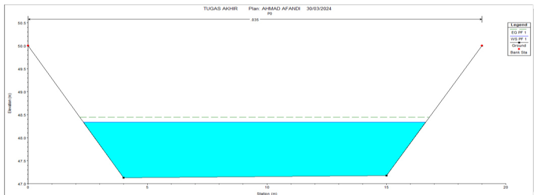
Gambar 4. Hasil Running Cross Section Qrencana STA P0 Sumber: Perhitungan Software HEC-RAS 5.0.1
