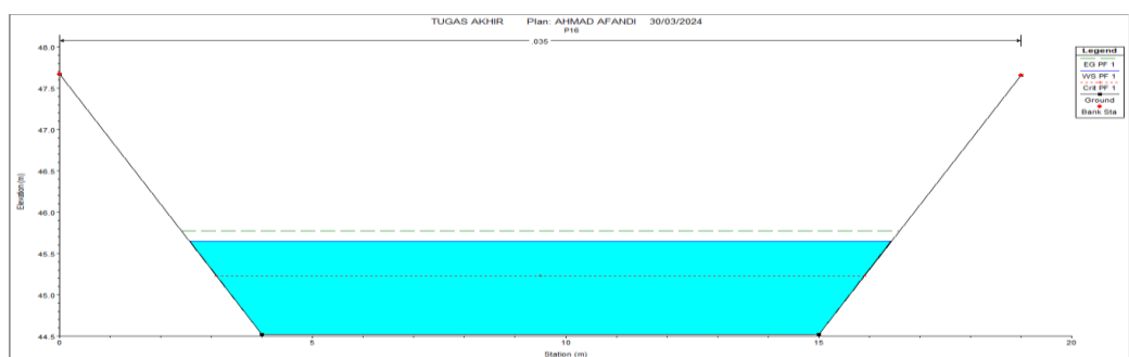
Gambar 5. Hasil Running Cross Section Qrencana STA P16 Sumber: Perhitungan Software HEC-RAS 5.0.1
