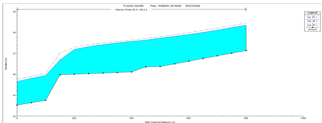
Gambar 6. Hasil Running Long Section Qrencana Sumber: Perhitungan Software HEC-RAS 5.0.1
